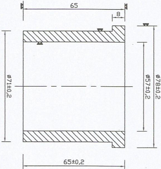
BUSH FOR LIFTING UNIT (PART NO. E150.35d)
